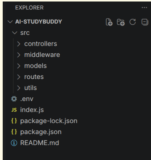
FIG 05 - FOLDER STRUCTURE
